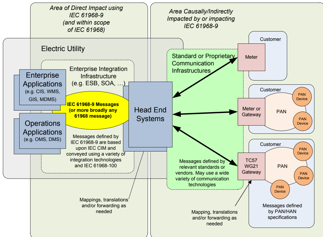
Figure 1 – IEC 61968-9 scope
