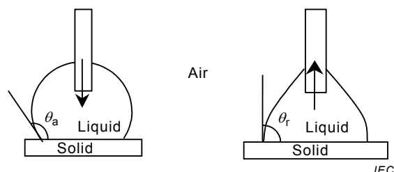
Figure 3 – Measurements of the advancing angle ( \theta_a ) and the receding angle ( \theta_r ) by adding or withdrawing water from a droplet
