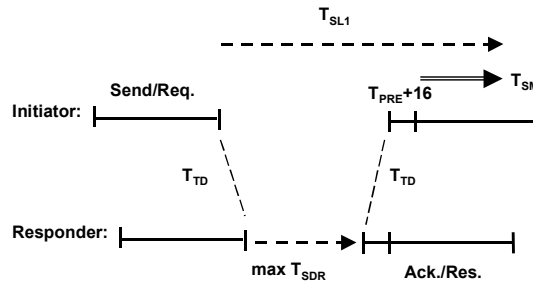
Figure 9 – Slot time T_{SL1}
