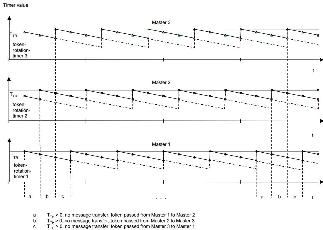
Figure C.2 – No usage of token holding time ( T_{TH} )
